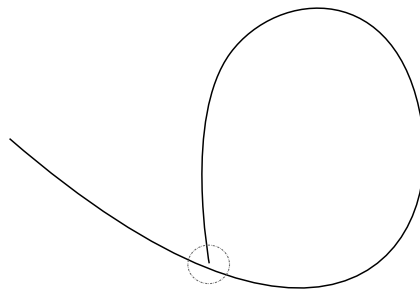
FIGURE 2. Prototypical example of a non-compact immersed submanifold that is not embedded.
