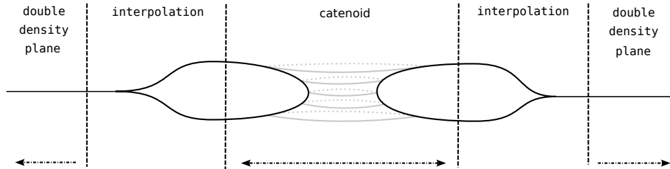
FIGURE 1. A catenoid patch such as the one described above.
