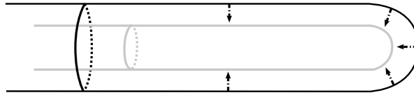
FIGURE 1. Two-dimensional cylindrical cap moving by mean curvature.
